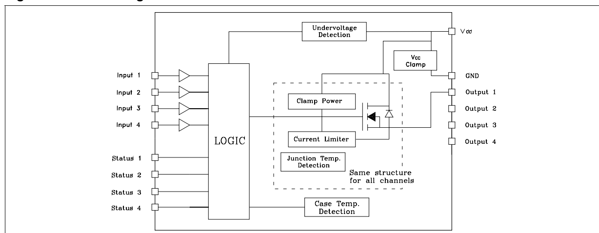
Figure 1. Block diagram
