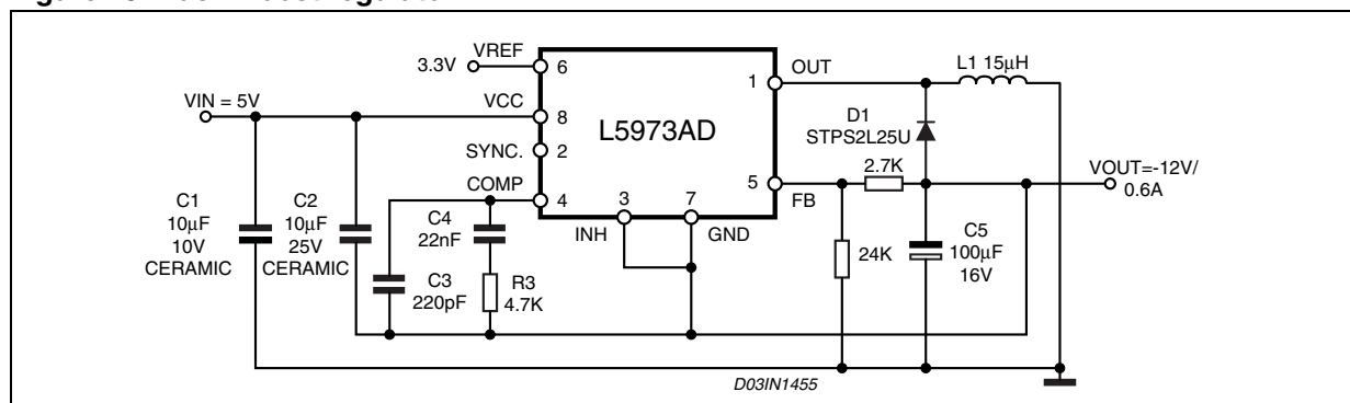
Figure 15. Buck-Boost regulator
