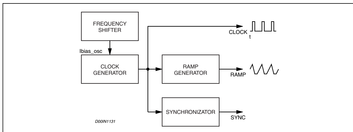
Figure 6. Oscillator Circuit
