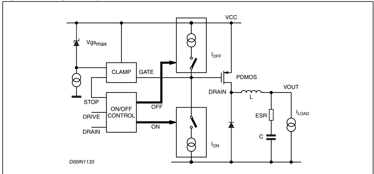
Figure 8. Driving Circuitry
