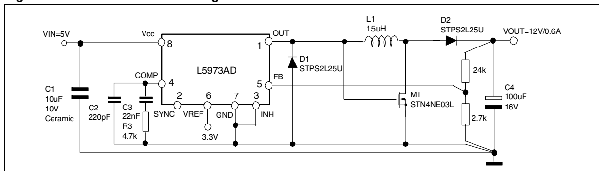
Figure 15. Buck-Boost regulator
