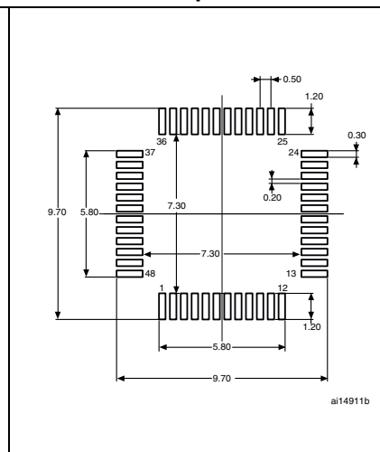
Figure 10. Recommended footprint (1)(2)
