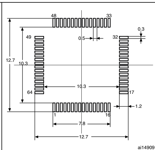
Figure 8. Recommended footprint (1)(2)
