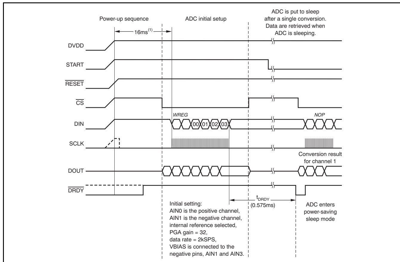
Figure 44. SPI Communication Sequence for Entering Sleep Mode After a Conversion
