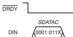
Figure 37. Stop Reading Data Continuously
