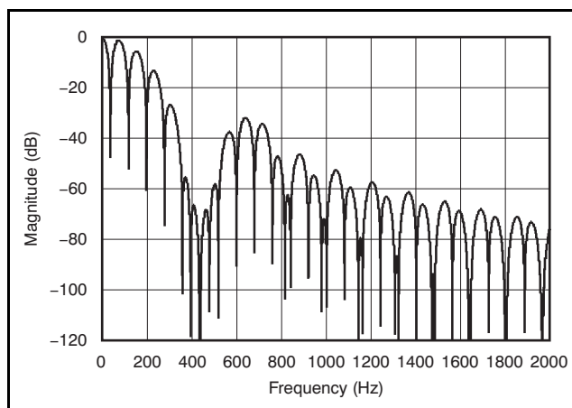
Figure 19. Filter Profile with Data Rate = 80SPS
