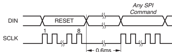
Figure 35. SPI Communication After an SPI Reset
