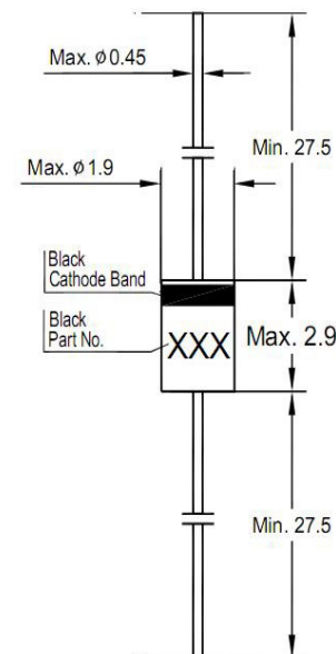
Glass Case DO-34 Dimensions in mm
