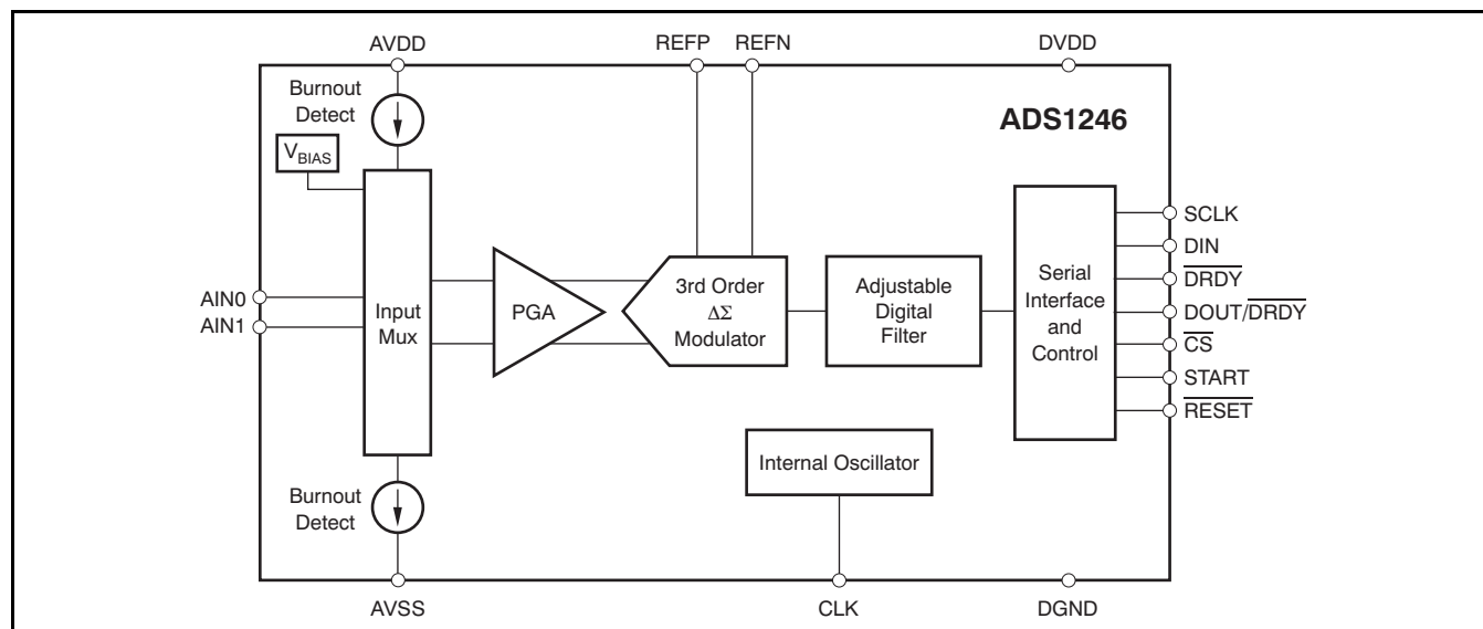
Figure 29. ADS1246 Diagram
