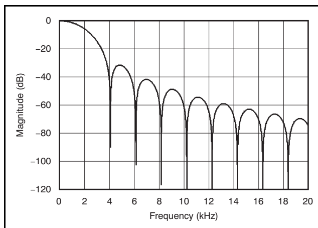
Figure 44. Filter Profile with Data Rate = 2kSPS
