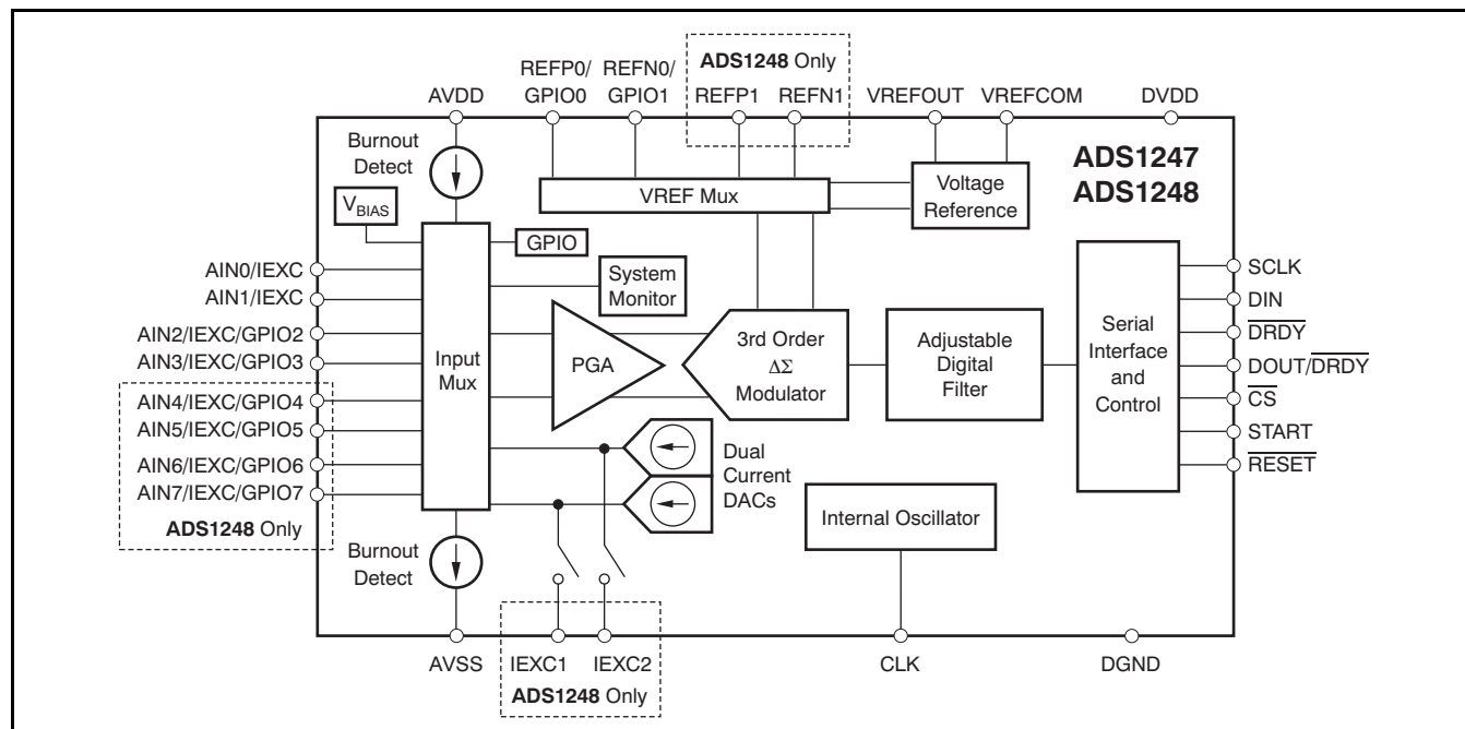
Figure 30. ADS1247, ADS1248 Diagram
