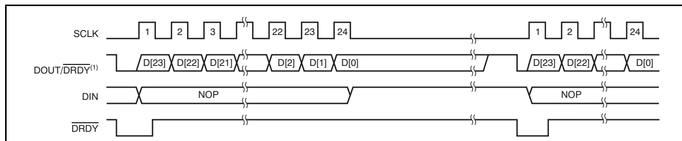
Figure 50. Data Retrieval with the DRDY MODE Bit = 1 (Enabled)
