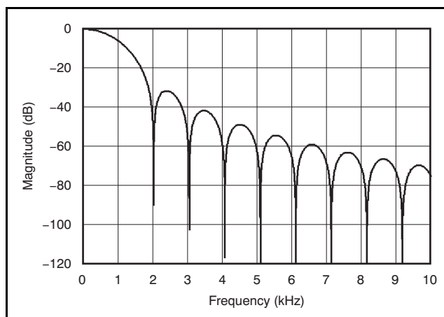
Figure 43. Filter Profile with Data Rate = 1kSPS
