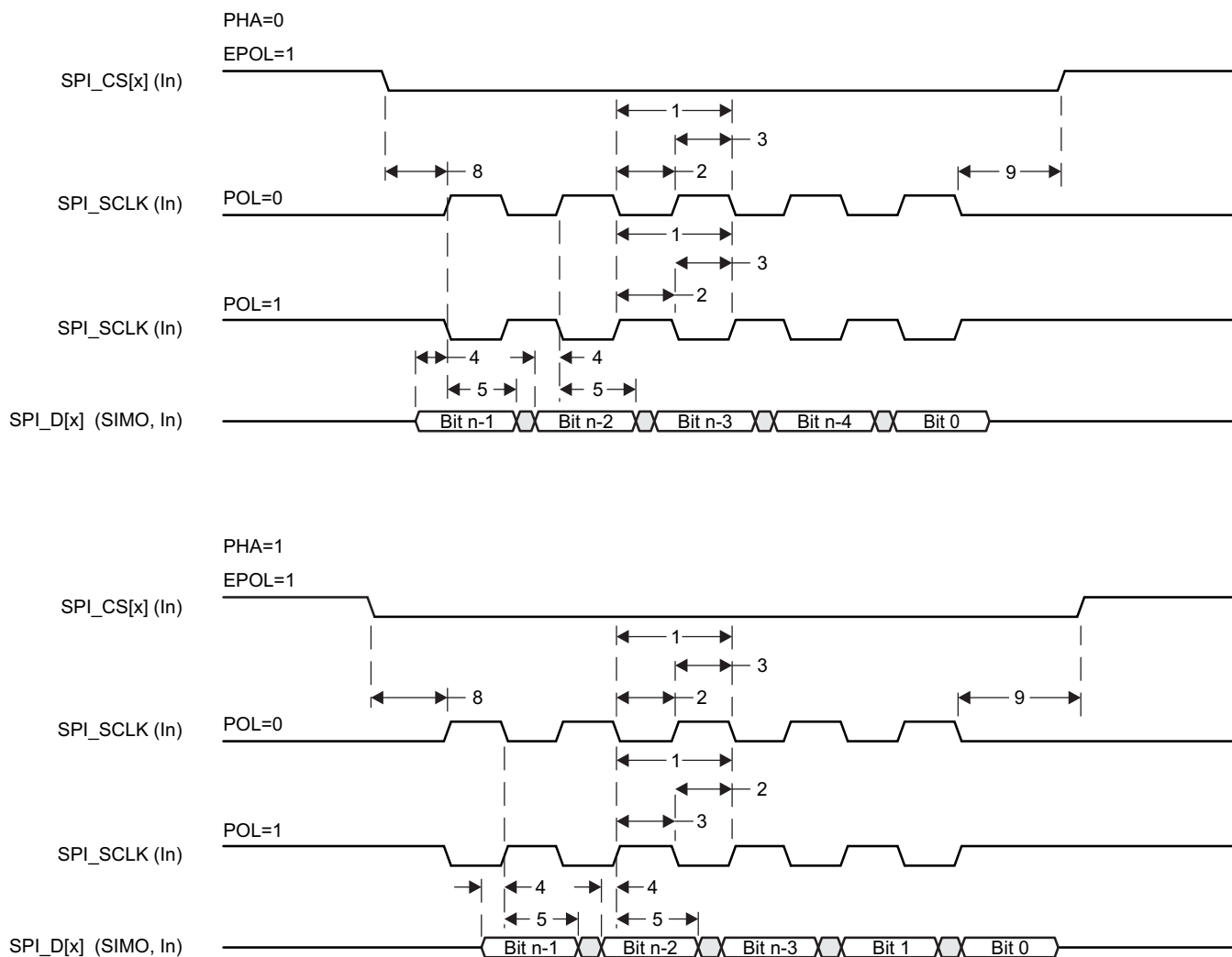
Figure 5-82. SPI Slave Mode Receive Timing
