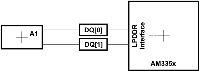
Figure 5-33. DQS[x] and DQ[x] Routing and Topology
