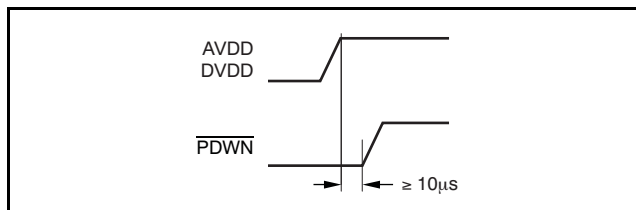
Figure 21. Power-Up Timing Sequence
