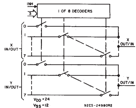
Fig. 2 - CD4097 functional diagram.
