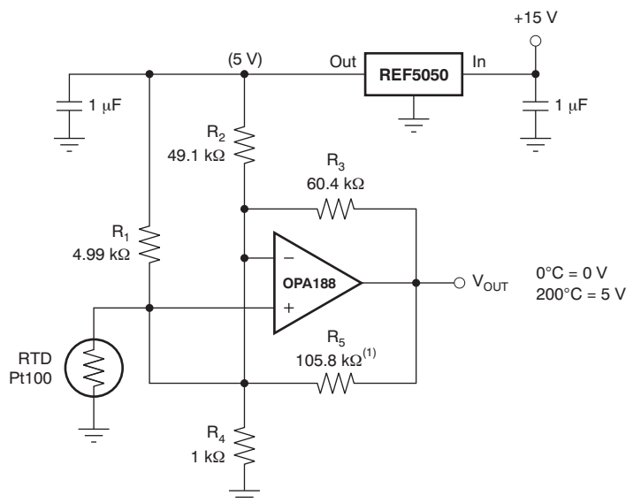
Figure 45. RTD Amplifier with Linearization
