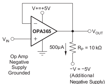
Figure 8. Swing-to-Ground
