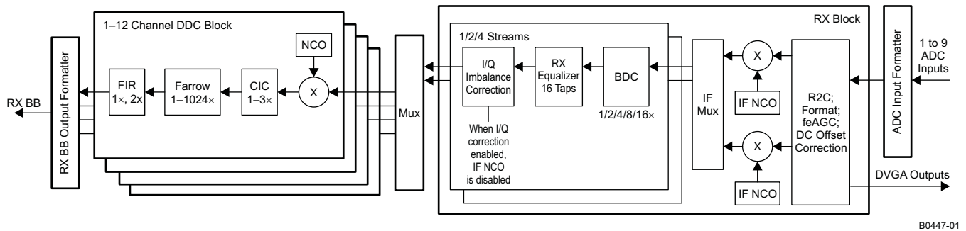
Figure 10. RX Functional Block Diagram
