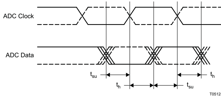
Figure 20. RX ADC LVDS Timing Specifications (RXA and RXB)
