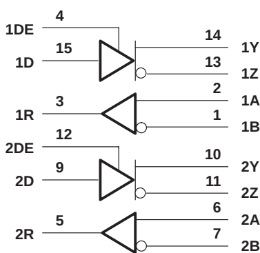
SN65C1168, SN75C1168
