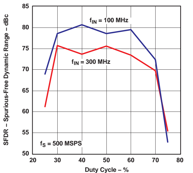
Figure 45. SFDR vs Clock Duty Cycle
