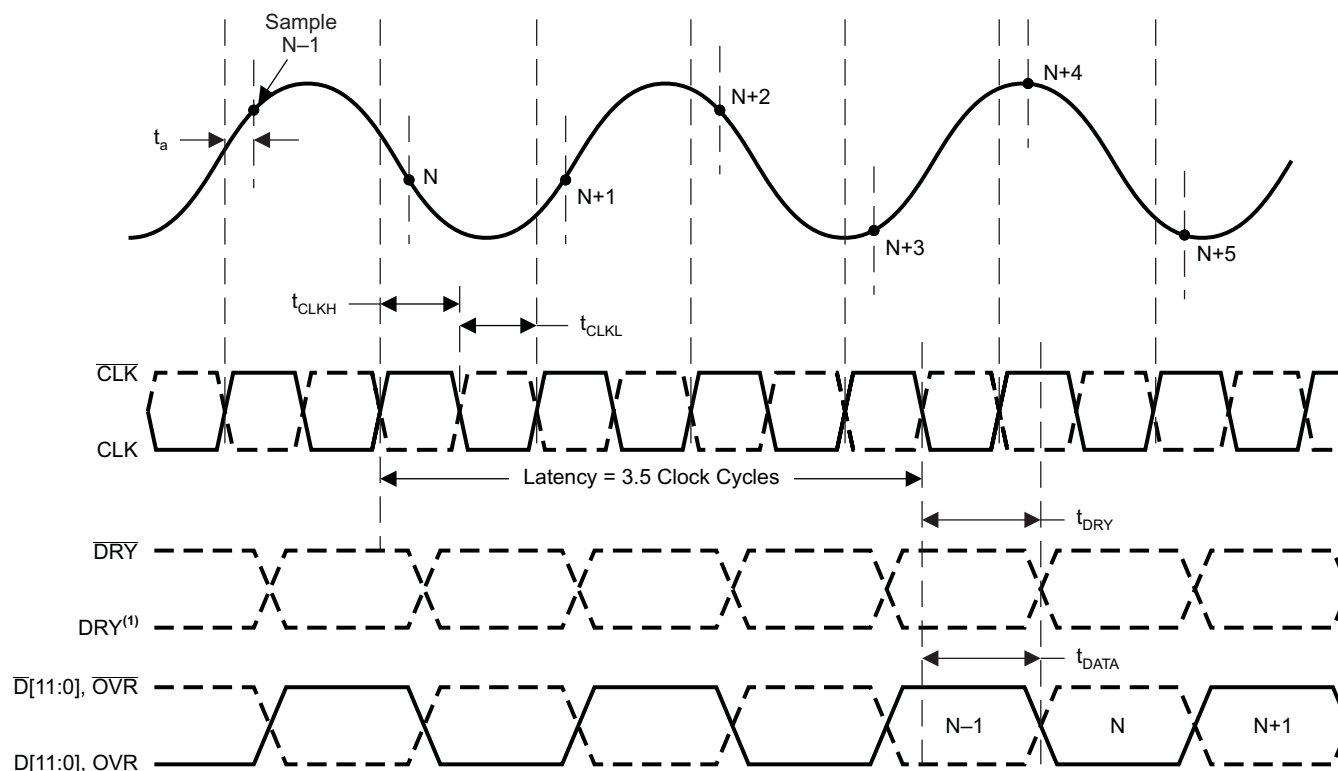
Figure 1. Timing Diagram
