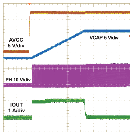
Figure 14. SuperCap Charge Cycle
