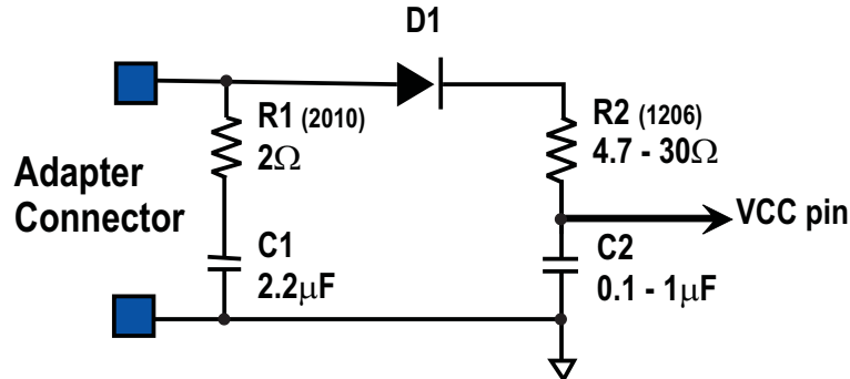
Figure 18. Input Filter
