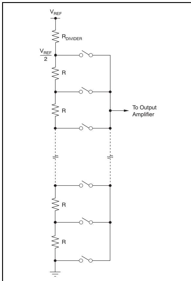
Figure 111. Resistor String
