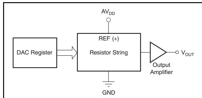
Figure 110. DACx311 Architecture
