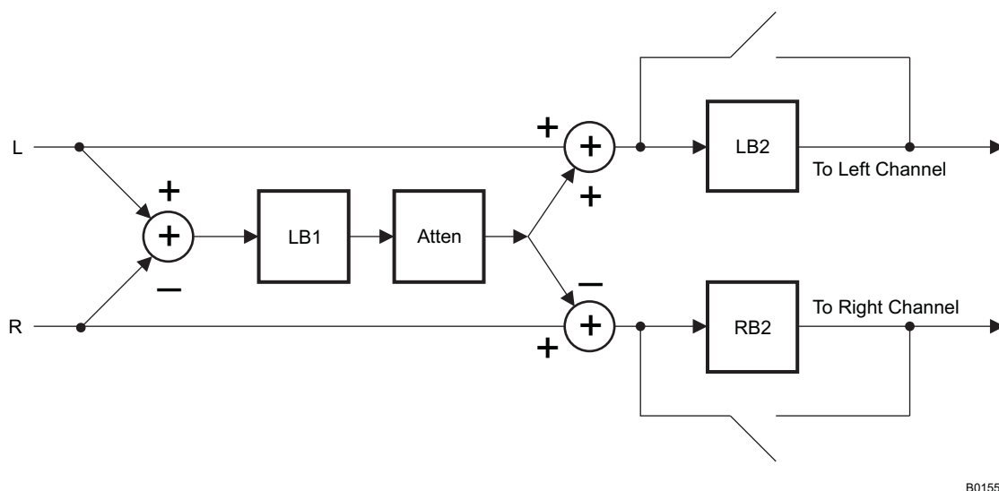
Figure 26. Architecture of the Digital Audio Processing When 3-D Effects Are Enabled
