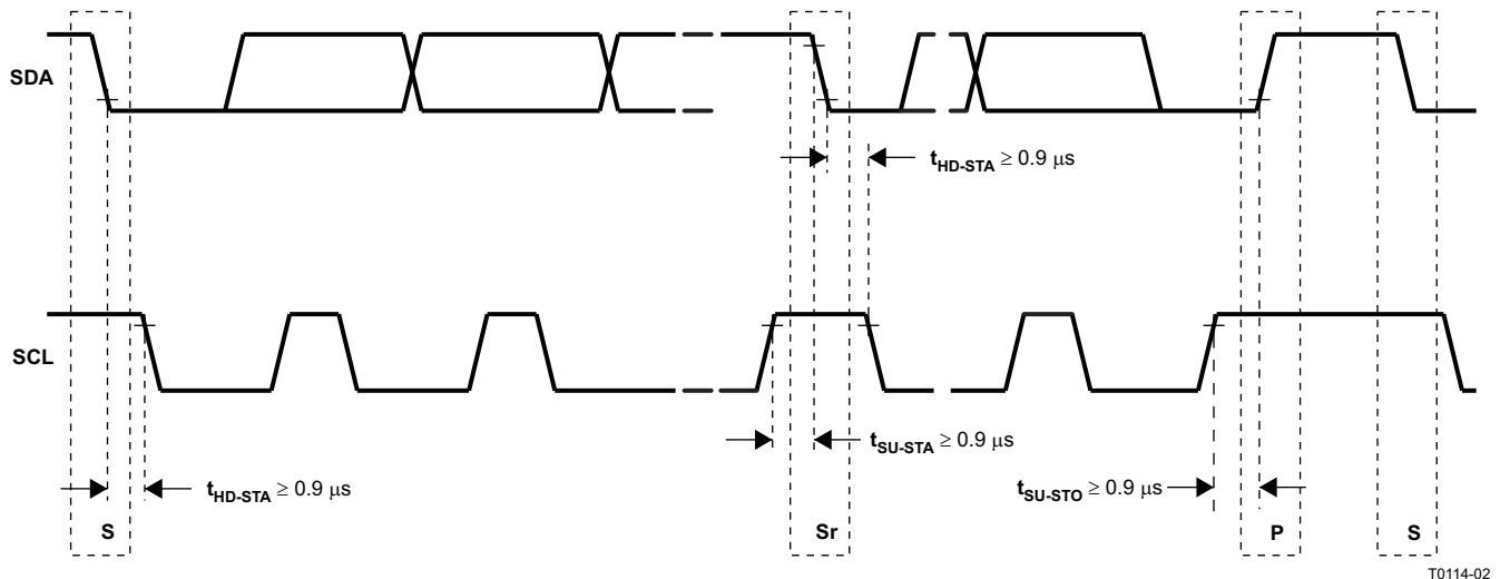
Figure 14. I²C Interface Timing
