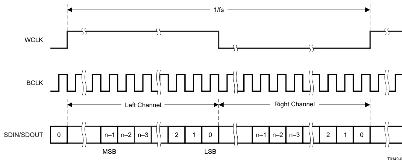
Figure 17. Right-Justified Serial Data Bus Mode Operation
