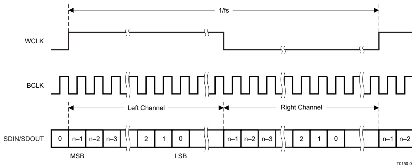
Figure 18. Left-Justified Serial Data Bus Mode Operation
