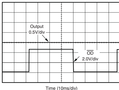
Figure 46. Output Signal During Toggle of \overline{\text{OD}}
