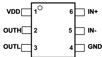
SOT-23 DBV (Top View)
