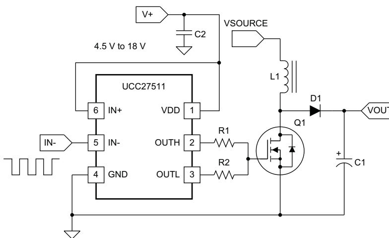
Figure 20. Using UCC27511 Inverting Input (IN+ is tied to VDD enable output)
