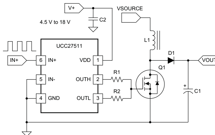
Figure 19. Using UCC27511 Non-Inverting Input (IN- is grounded to enable output)
