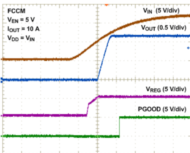
Time (2 ms/div) Figure 30. UVLO Start-Up
