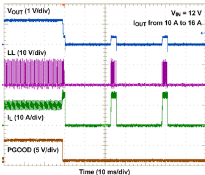
Figure 37. Overcurrent Protection
