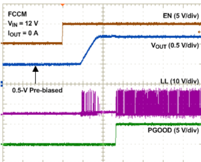
Time (1 ms/div) Figure 28. Pre-Bias Start-Up
