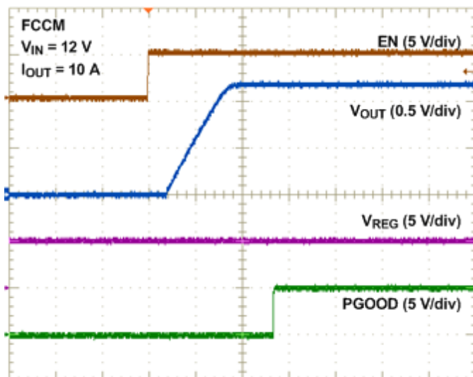
Time (1 ms/div) Figure 27. Start-Up
