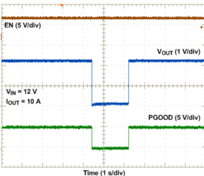
Figure 38. Over-temperature Protection
