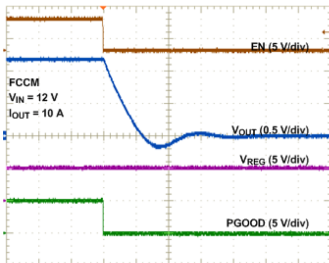
Time (40 μs/div) Figure 29. Shutdown
