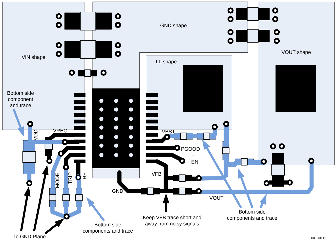
Figure 45. Layout Recommendation
