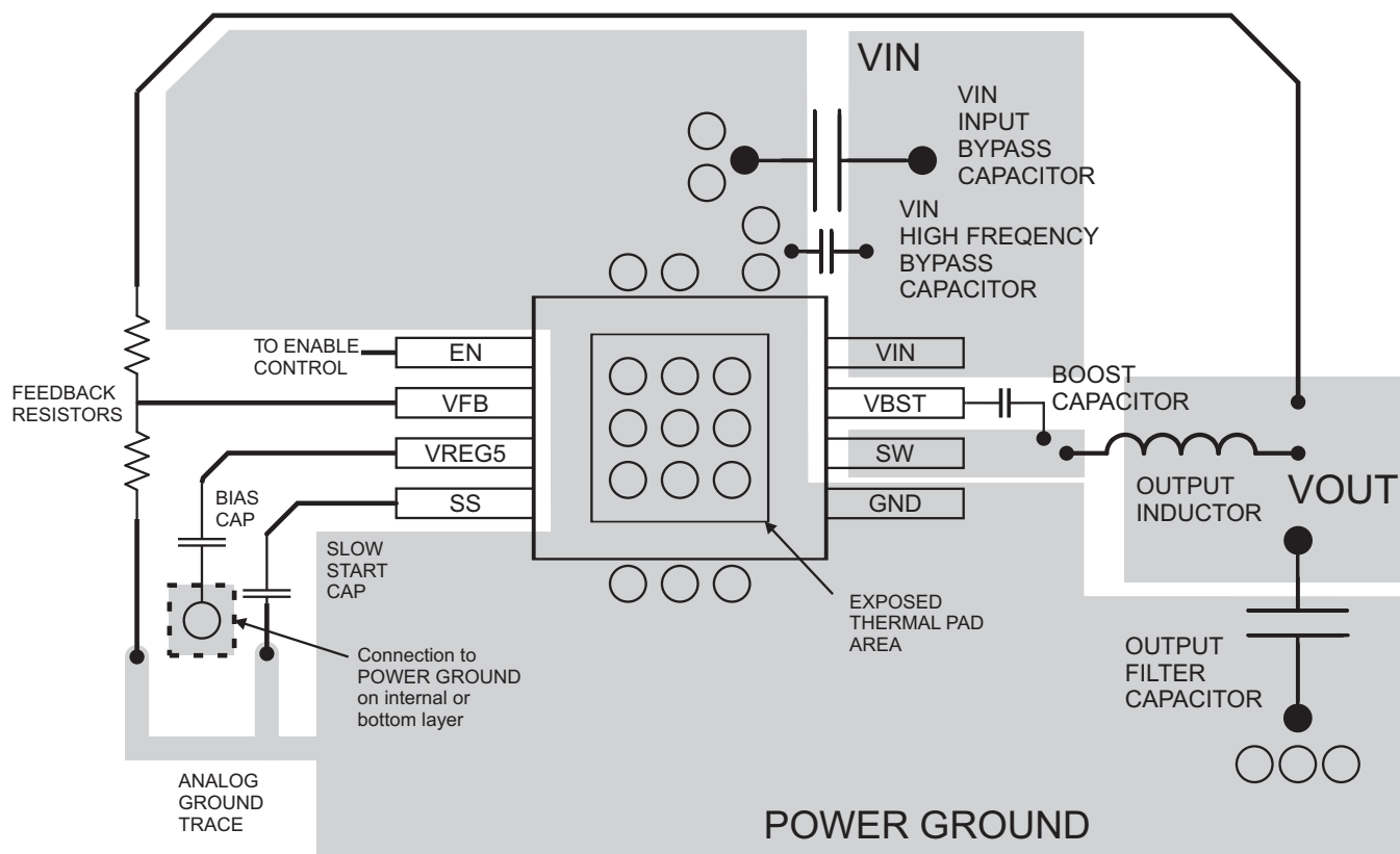
Figure 19. PCB Layout
