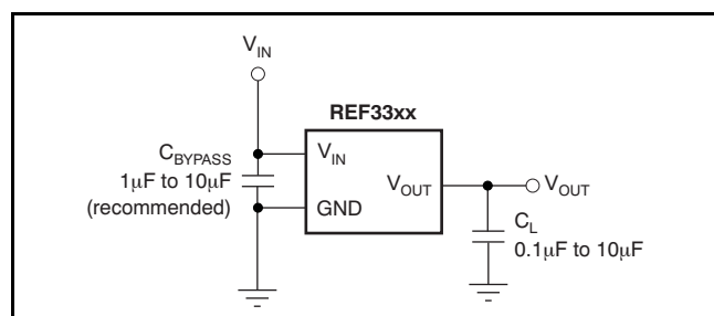
Figure 18. Basic Connections
