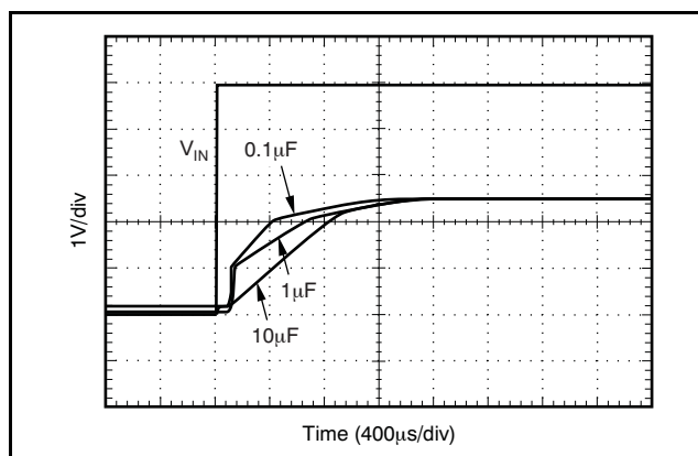
Figure 19. Start-Up Time
