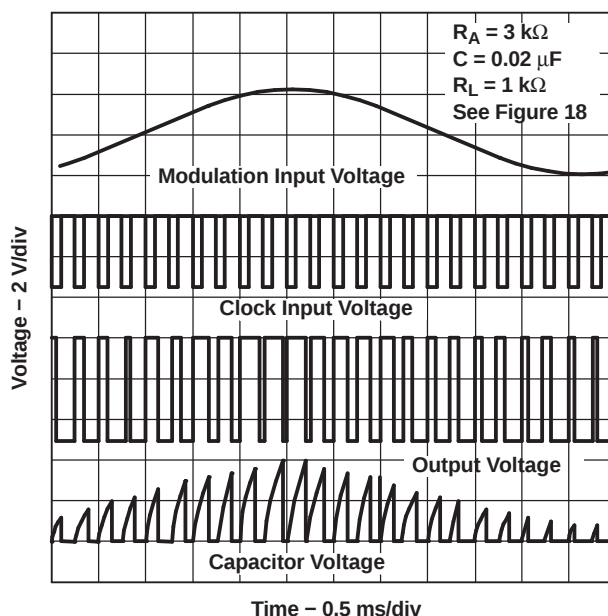
Figure 19. Pulse-Width-Modulation Waveforms
