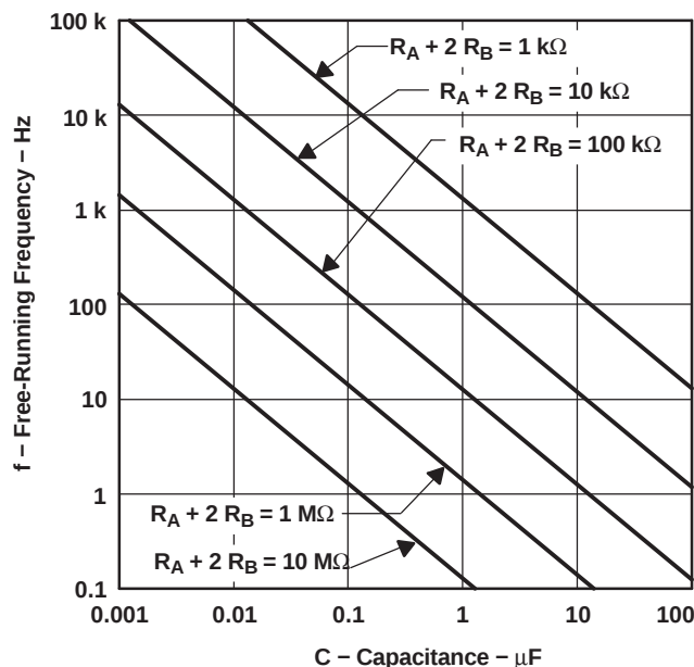
Figure 14. Free-Running Frequency
