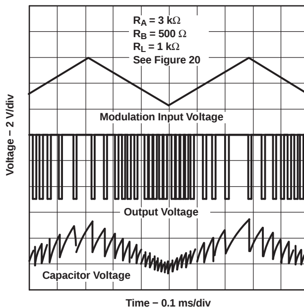
Figure 21. Pulse-Position-Modulation Waveforms
