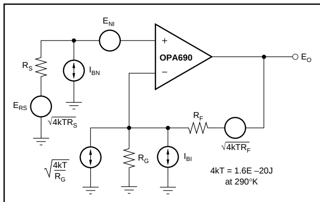
FIGURE 11. Op Amp Noise Analysis Model.
