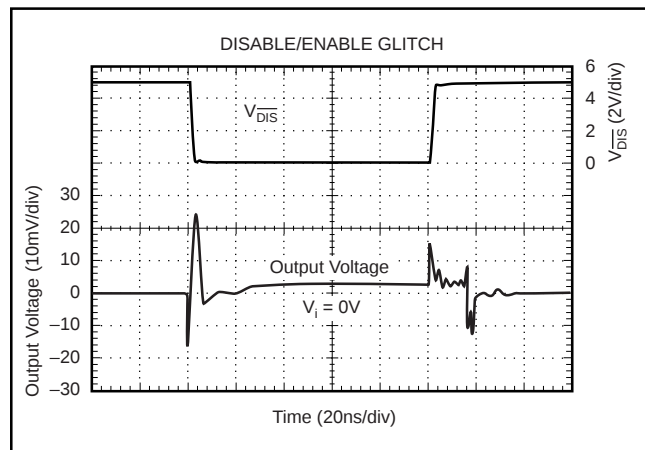
FIGURE 14. Disable/Enable Glitch.
