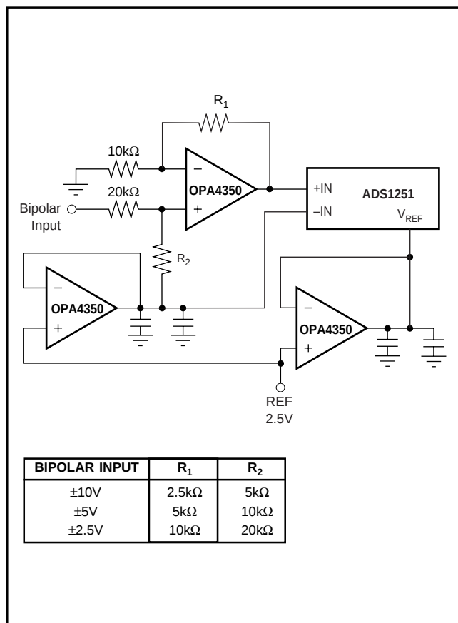
FIGURE 1. Level-Shift Circuit for Bipolar Input Ranges.
