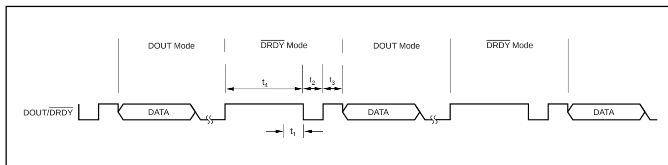
FIGURE 11. DOUT/DRDY Partitioning.
