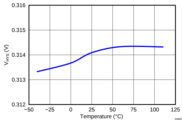
Figure 5. Hysteresis V_{HYS} vs. Temperature
