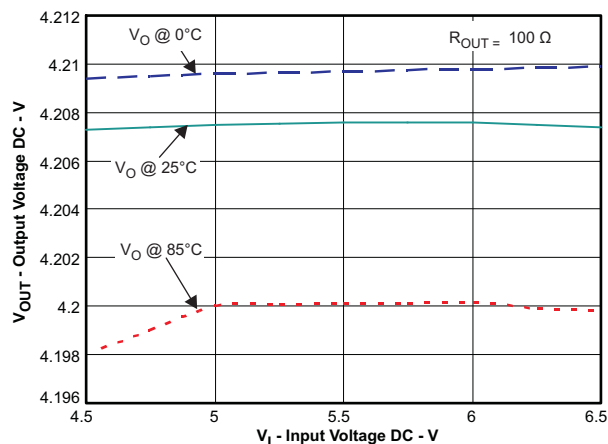
Figure 16. Line Regulation
