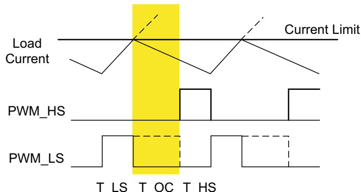
Figure 7. Cycle-by-Cycle Operation with Low Side OC (dashed line: normal operation; solid line: CBC event)
