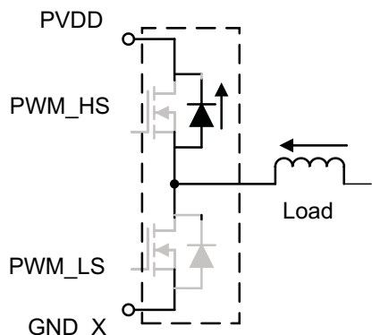
Figure 7. Cycle-by-Cycle Operation with Low Side OC (dashed line: normal operation; solid line: CBC event)
