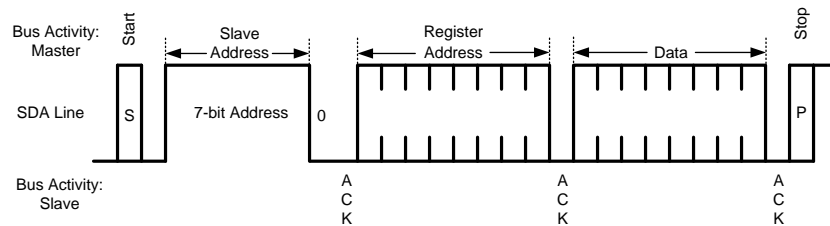
Figure 31. Write Byte
