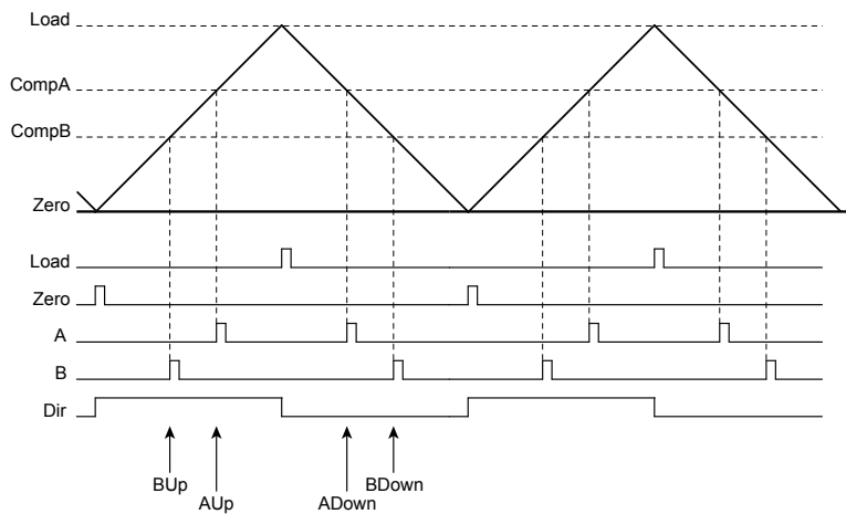
Figure 19-4. PWM Count-Up/Down Mode
