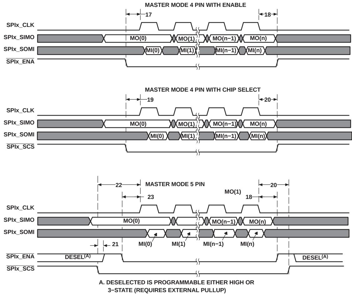
Figure 5-39. SPI Timings—Master Mode (4-Pin and 5-Pin)
