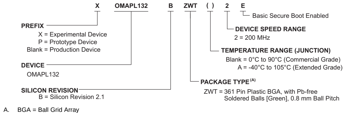
Figure 6-1. Device Nomenclature
