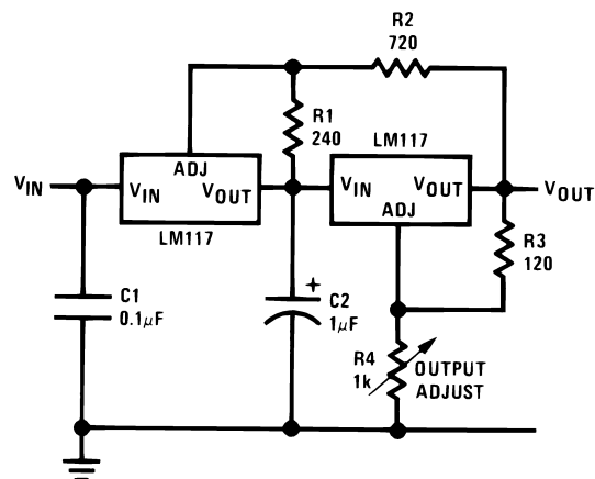
Figure 53. Tracking Preregulator
