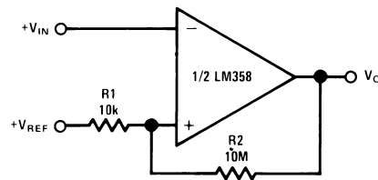
Figure 33. Comparator with Hysteresis
