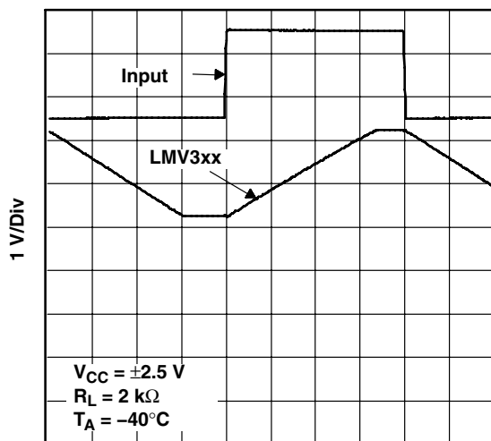
1 μs/Div Figure 29
