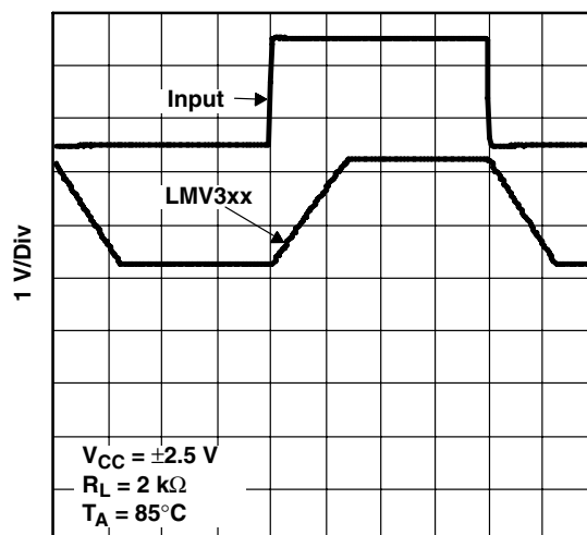
1 μs/Div Figure 28
