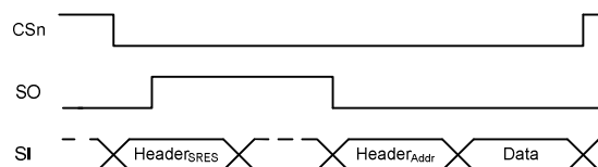
Figure 12: SRES Command Stroke
