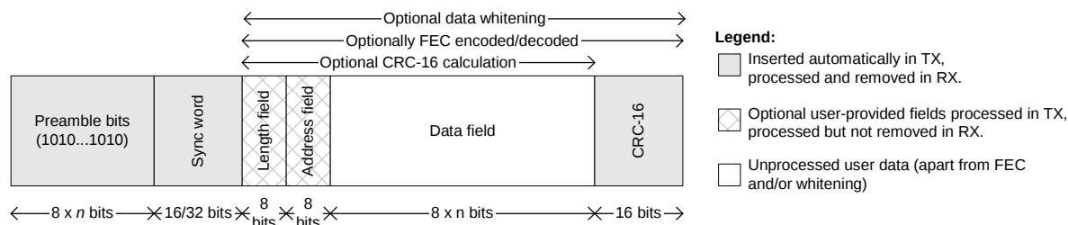
Figure 15: Packet Format
