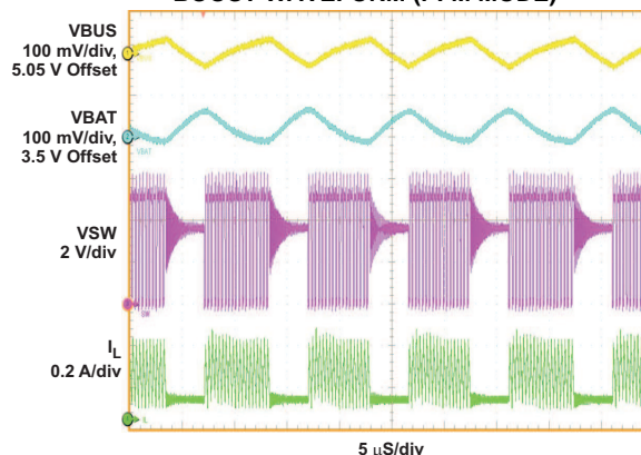
Figure 12. VBUS = 5.05 V, VBAT = 3.5V, IBUS = 42 mA
