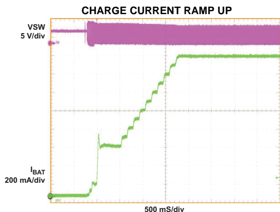
Figure 7. \text{Vin} = 5\text{ V} , \text{VBAT} = 3.2\text{ V} , No Input Current Limit, \text{I}_{\text{CHG}} = 1550\text{ mA}
