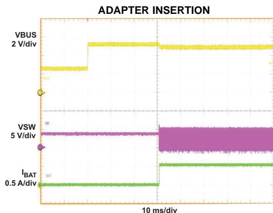
Figure 3. \text{VBUS} = 0\text{-}5\text{ V} , \text{lin\_limit} = 500\text{ mA} , \text{Voreg} = 4.2\text{ V} , \text{VBAT} = 3.5\text{ V} , \text{I}_{\text{CHG}} = 550\text{ mA} , 32S mode
