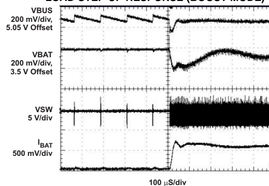
Figure 14. VBUS = 5.05, VBAT = 3.5V, IBUS = 0-360 mA
