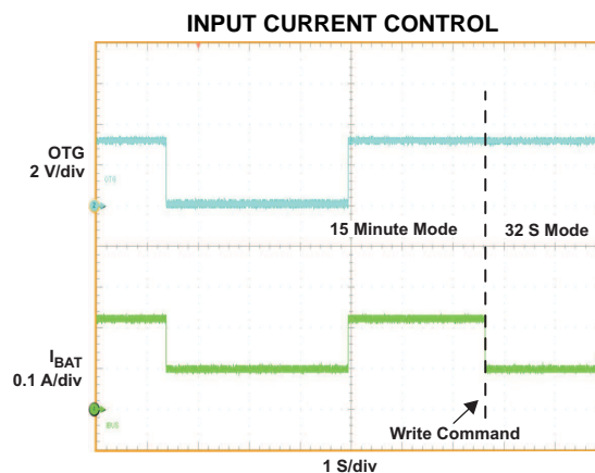
Figure 8. \text{VBUS} = 5\text{ V} , \text{VBAT} = 3.1\text{ V} , \text{lin\_limit} = 100/500\text{ mA} , (OTG Control, 15 Minute Mode), \text{lin\_limit} = 100\text{ mA} ( \text{I}^2\text{C} Control, 32 Second Mode)
