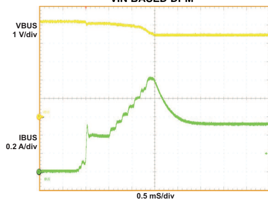
Figure 9. VBUS = 5 V at 500 mA, VBAT = 3.5V, ICHG = 1550 mA, VIN_DPM = 4.52 V
