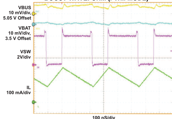
Figure 11. VBUS = 5.05 V, VBAT = 3.5V, IBUS = 217 mA
