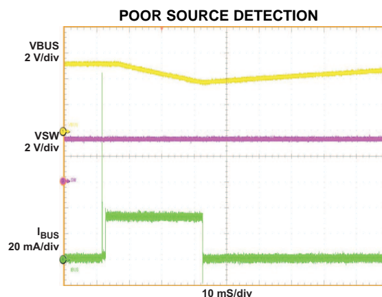
Figure 6. \text{VBUS} = 5\text{ V} at 8\text{ mA} , \text{VBAT} = 3.2\text{ V} , \text{lin\_limit} = 100\text{ mA} , \text{I}_{\text{CHG}} = 550\text{ mA}
