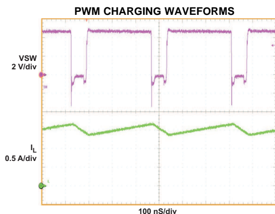
Figure 5. \text{VBUS} = 5\text{ V} , \text{VBAT} = 2.6\text{ V} , \text{Voreg} = 4.2\text{ V} , \text{I}_{\text{CHG}} = 1550\text{ mA}
