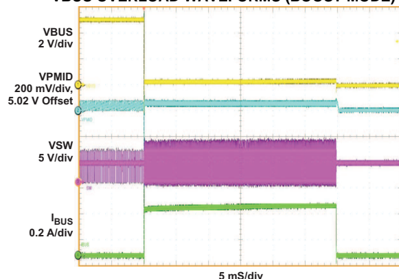
Figure 13. VBUS = 5.05 V, VBAT = 3.5V, RLOAD (at VBUS) = 1KΩ to 0.5Ω
