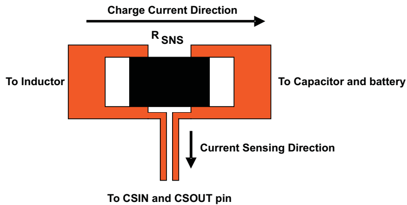
Figure 36. Sensing Resistor PCB Layout
