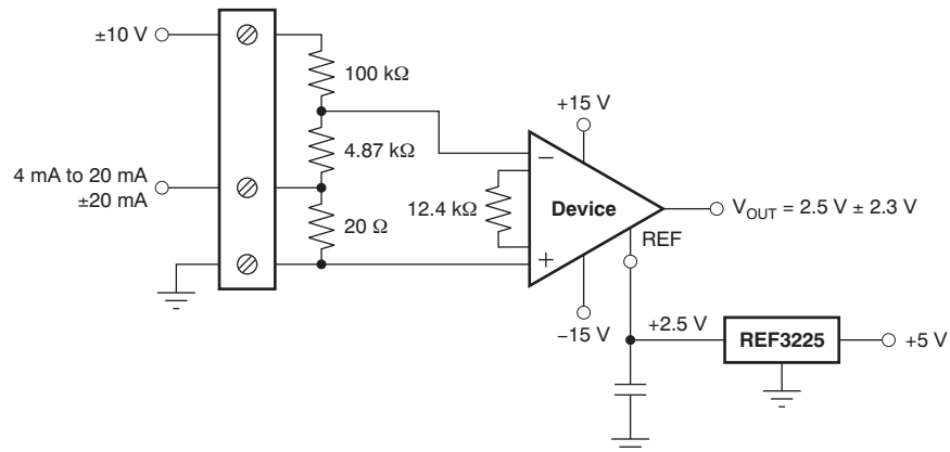
Figure 65. ±10-V, 4-mA to 20-mA PLC Input
