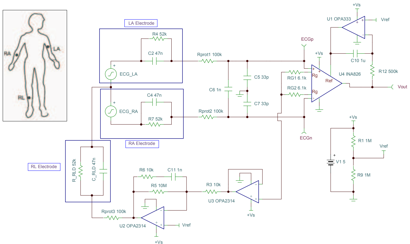
Figure 67. ECG Circuit
