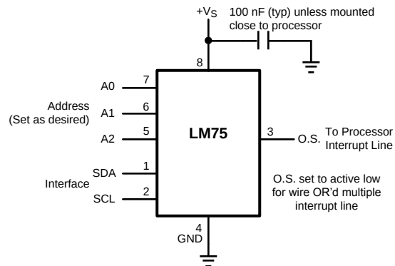
Figure 2. Typical Application
