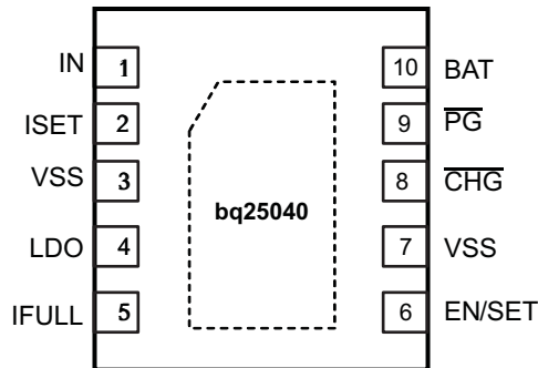
10-Pin 2mm × 3mm DFN (TOP VIEW)
