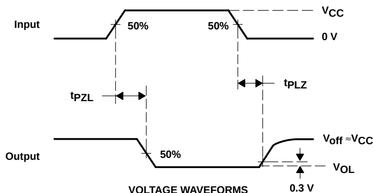
VOLTAGE WAVEFORMS
