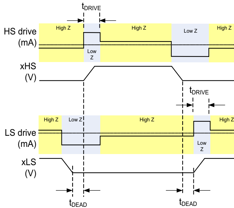
Figure 6. Pre-Drivers
