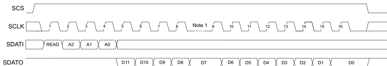
Figure 11. Read Operation
