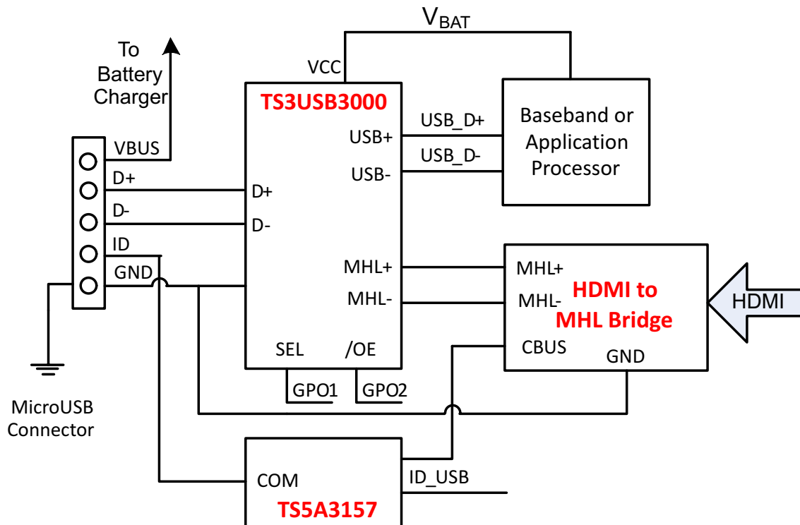
Figure 1. Typical TS3USB3000 Application
