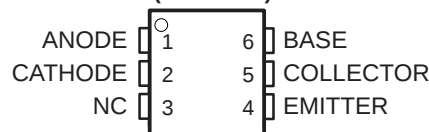
DCJ † OR 6-TERMINAL DUAL-IN-LINE PACKAGE (TOP VIEW)
