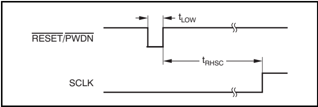
Figure 47. \overline{\text{RESET/PWDN}} Timing
