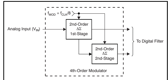
Figure 32. Fourth-Order Modulator
