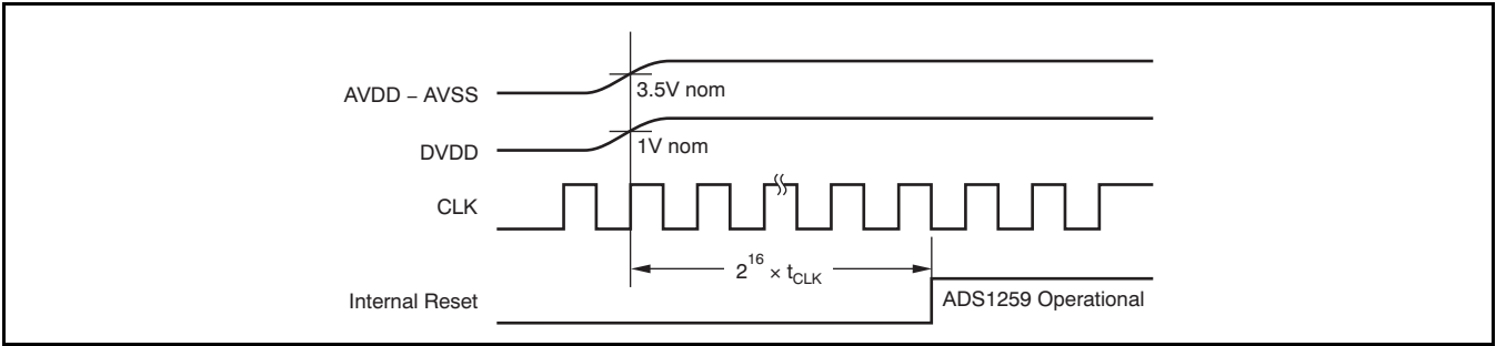
Figure 48. Power-On Sequence
