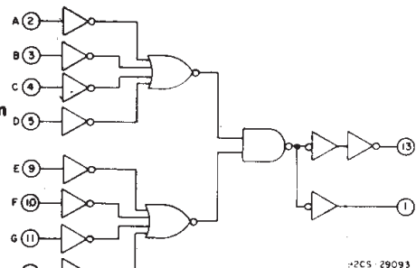
Fig. 1 – Logic diagram.
