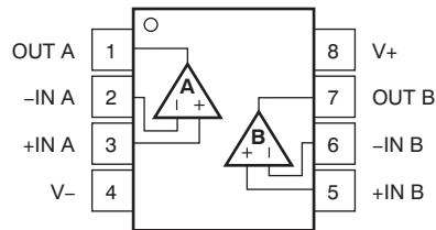
OPA2188 D, DGK PACKAGES (SO-8, MSOP-8) (TOP VIEW)
