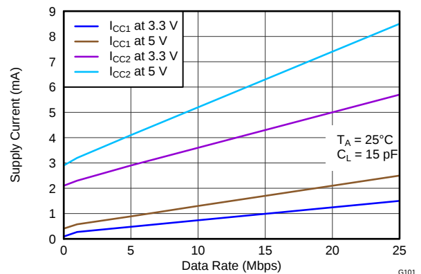
Figure 13. ISO7640FC Supply Current For All Channels vs Data Rate
