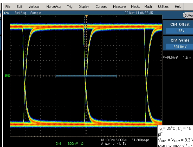
Figure 28. C-Grade Typical Eye Diagram at 25 Mbps, 3.3 V Operation
