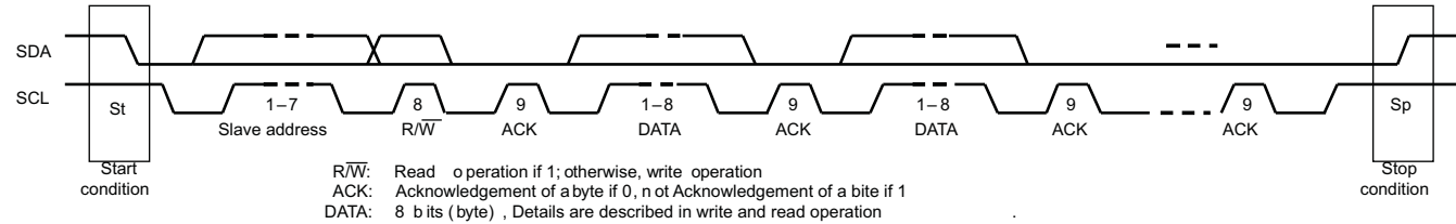
Figure 40. I²C Packet Protocol
