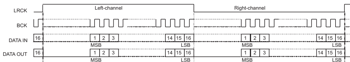
Figure 12. Audio Data Input/Output Format
