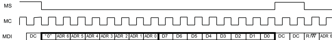
Figure 37. Register Write Operation
