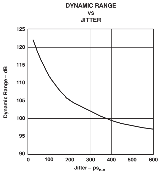
Figure 35. Jitter Dependence ( \times 64 Oversampling)
